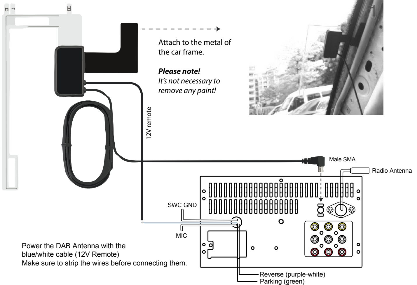
Stick the transparent part of the antenna on the windshield and put the black part on the metal frame.
